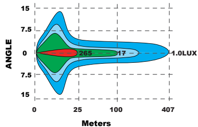
COMBO BEAM(ECE-ref.37.5)
