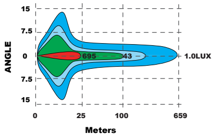
COMBO BEAM(off-road)
